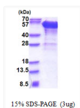
SDS-PAGE gel of recombinant human Dynactin Subunit 2 DCTN2 protein under reducing conditions
