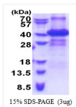
SDS-PAGE gel of recombinant human ING2 protein under reducing conditions stained with Coomassie blue
