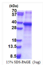
SDS-PAGE gel of recombinant human RPS2 protein 3µg under reducing conditions stained with Coomassie blue
