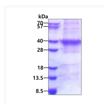
SDS-PAGE gel showing recombinant human UBC3B UBE2R2 protein under reducing conditions Coomassie stain
