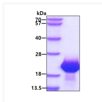
SDS-PAGE of recombinant human FAM107B protein under reducing conditions stained with Coomassie blue
