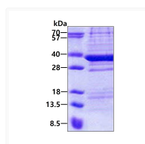
SDS-PAGE gel of recombinant human TPGS2 protein under reducing conditions stained with Coomassie blue
