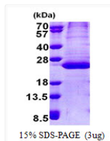
SDS-PAGE gel of recombinant human DESI1 protein under reducing conditions stained with Coomassie blue
