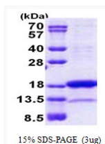
SDS-PAGE gel of recombinant human PNRC2 protein under reducing conditions
