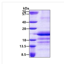
SDS-PAGE gel of recombinant human GATC protein under reducing conditions stained with Coomassie blue
