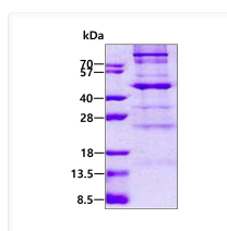
SDS-PAGE of recombinant human C1GalT1/C1GalT1C1 protein under reducing conditions
