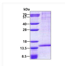
Recombinant human RAB8B protein SDS-PAGE gel 3 µg Coomassie blue stain
