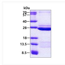
SDS-PAGE gel of recombinant human FAM50A protein 3µg under reducing conditions stained with Coomassie blue
