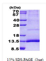
SDS-PAGE gel of recombinant human CST11 protein under reducing conditions stained with Coomassie blue
