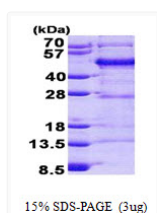
SDS-PAGE gel of recombinant human FBLIM1 protein 3µg under reducing conditions stained with Coomassie blue
