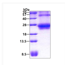
SDS-PAGE gel of recombinant human RhoQ protein 3µg under reducing conditions Coomassie stain
