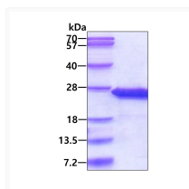
SDS-PAGE gel of recombinant human HN1 protein 3µg under reducing conditions Coomassie blue stain
