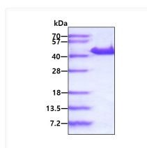
SDS-PAGE gel showing recombinant human YOD1 protein 3µg under reducing conditions with Coomassie blue stain
