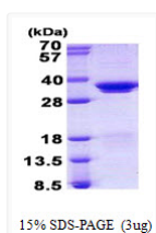
SDS-PAGE gel of recombinant human SFRS1 protein under reducing conditions stained with Coomassie blue
