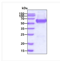
SDS-PAGE of recombinant human ALT2 GPT2 protein under reducing conditions with Coomassie blue stain
