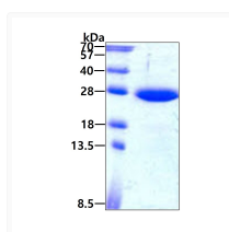
SDS-PAGE gel of recombinant human SAR1B protein 3µg under reducing conditions Coomassie blue stain
