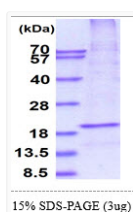
SDS-PAGE gel of recombinant human Fas Ligand FASLG protein under reducing conditions stained with Coomassie blue
