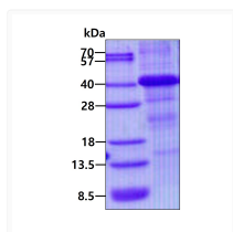
SDS-PAGE gel showing recombinant human HFE protein 3µg under reducing conditions stained with Coomassie blue
