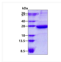
SDS-PAGE gel of recombinant human HEBP1 protein stained with Coomassie blue
