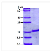
SDS-PAGE gel of recombinant human IRGM protein under reducing conditions Coomassie blue stain
