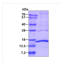
SDS-PAGE gel of recombinant human NDUF5 protein under reducing conditions stained with Coomassie blue
