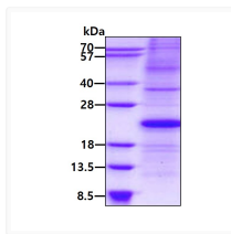
SDS-PAGE gel of recombinant human p21 CIP1 CDKN1A protein under reducing conditions
