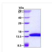
SDS-PAGE gel of recombinant human SH3BGRL3 protein Coomassie blue stain reducing conditions
