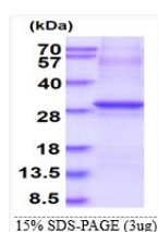
SDS-PAGE gel of recombinant human 2B4/CD244 protein under reducing conditions
