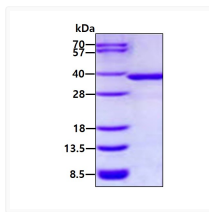
SDS-PAGE gel of recombinant human NMRAL1 protein 3µg reducing conditions Coomassie blue stain
