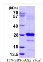
Recombinant human PLDN protein SDS-PAGE gel under reducing conditions
