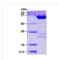
SDS-PAGE of recombinant human DARS protein under reducing conditions Coomassie blue stain
