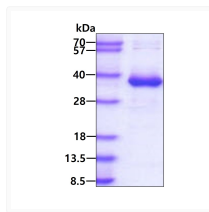
SDS-PAGE gel of recombinant human CYB5R3 protein 3µg under reducing conditions stained with Coomassie blue
