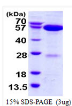
SDS-PAGE gel of recombinant human APPBP1/NAE1 protein under reducing conditions stained with Coomassie blue
