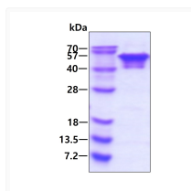
SDS-PAGE gel showing recombinant human NEIL1 protein 3µg under reducing conditions Coomassie blue stain
