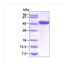
Recombinant human LCMT1 protein SDS-PAGE gel 3µg reducing conditions Coomassie blue stain
