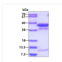
SDS-PAGE gel of recombinant human HDHD2B/LHPP protein 3µg reducing conditions Coomassie blue stain
