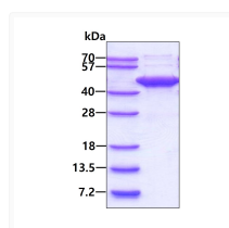
SDS-PAGE gel of recombinant human p38 beta MAPK11 protein under reducing conditions stained with Coomassie blue
