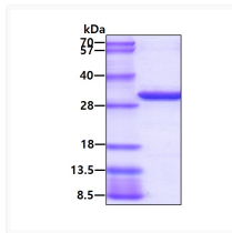
SDS-PAGE gel of recombinant human PSMA3 protein 3µg reducing conditions Coomassie blue stain
