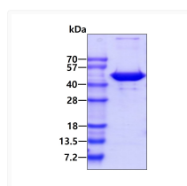
Recombinant human IDH1 protein SDS-PAGE gel 3µg Coomassie blue stain reducing conditions
