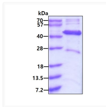
Recombinant human ACADL protein SDS-PAGE gel under reducing conditions stained with Coomassie blue
