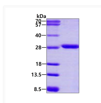
SDS-PAGE gel of recombinant human PSMA2 protein 3µg under reducing conditions stained with Coomassie blue
