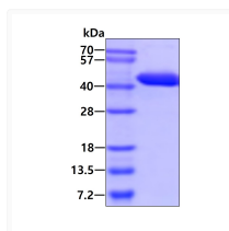
SDS-PAGE gel showing recombinant human GNAI1 protein 3µg under reducing conditions with Coomassie blue stain
