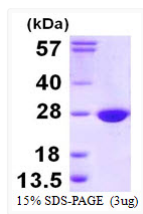
SDS-PAGE gel of recombinant human COX4NB protein under reducing conditions stained with Coomassie blue
