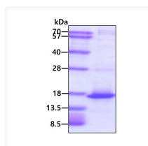
SDS-PAGE gel of recombinant human MYL5 protein 3µg under reducing conditions Coomassie blue stain
