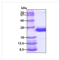
SDS-PAGE gel showing recombinant human CRYGD protein under reducing conditions Coomassie blue stain
