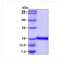
SDS-PAGE gel of recombinant human Ubch5b/UBE2D2 protein under reducing conditions
