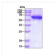
SDS-PAGE gel of recombinant human ATF4 protein 3µg under reducing conditions stained with Coomassie blue
