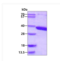
SDS-PAGE gel of recombinant human ACY3 protein under reducing conditions stained with Coomassie blue
