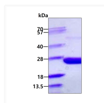
SDS-PAGE gel of recombinant E. coli PPA protein under reducing conditions Coomassie blue stain
