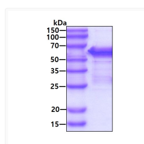
SDS-PAGE gel of recombinant human SHC1 protein 3µg under reducing conditions Coomassie blue stained
